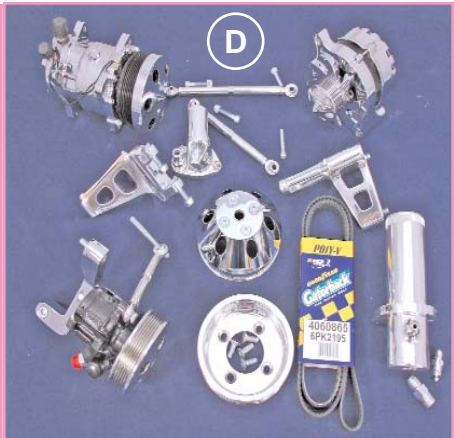
351 Windsor w/ Short Reverse Flow Water Pump & Pass/PS 65 AMP
