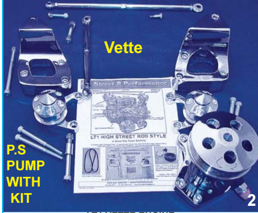
LT1 HIGH STREET ROD STYLE 30 Power Steering
