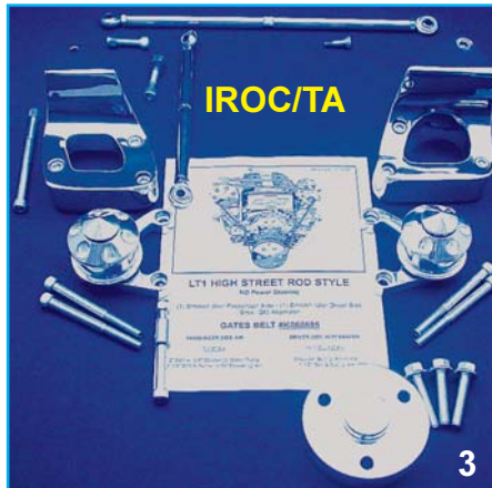
LT1 HIGH STREET ROD STYLE 40 Power Steering
