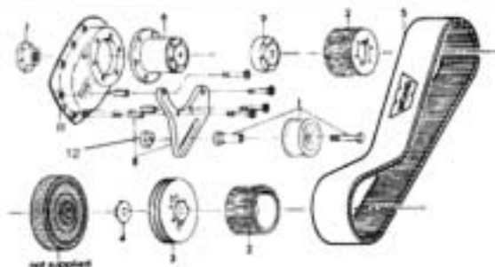
Components Parts List for 8mm Pitch Drives
